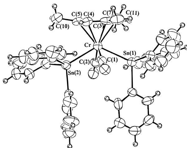
Figure 1. Diagram of the structure of (\eta^6\text{-C}_6\text{H}_3(\text{CH}_3)_3)\text{Cr}(\text{CO})_2(\text{SnPh}_3)_2 .
