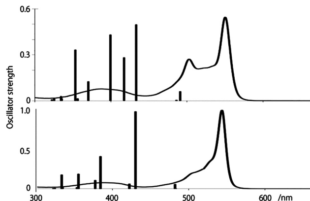
Fig. 8 TD-DFT results of syn -6a (upper) and anti -6a (lower) with UV-vis spectra.
