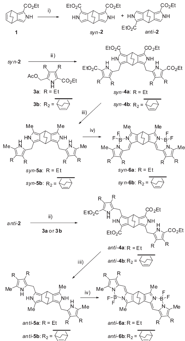
Scheme 1 Reagents, conditions, and yields: (i) ref. 11. (ii) 3 , p -TsOH, AcOH, rt; syn - 4a , 54%; syn - 4b , 61%; anti - 4a , 73%; and anti - 4b , 72%. (iii) LiAlH 4 , THF, reflux; syn - 5a , 96%; syn - 5b , 65%; anti - 5a , 93%; and anti - 5b , 82%. (iv) chloranil, BF 3 ·OEt 2 , (i-Pr) 2 EtN, CH 2 Cl 2 , rt; syn - 6a , 36%; syn - 6b , 70%; anti - 6a , 53%; and anti - 6b , 82%.
