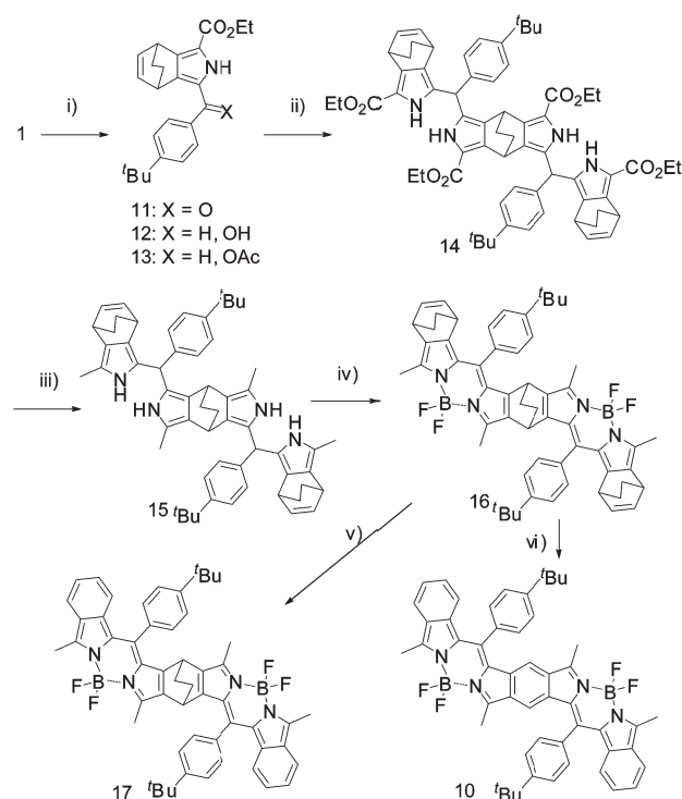
Scheme 2 (i) 4- tert -Butylbenzoic acid, TFAA, TFA, rt; 77%; \text{NaBH}_4 , THF–MeOH, rt; 95%; \text{Ac}_2\text{O} , DMAP, \text{CH}_2\text{Cl}_2 , rt; 99%. (ii) anti -2, p\text{TSA} , AcOH, rt; 99%; (iii) \text{LiAlH}_4 , THF, reflux; 86%. (iv) DDQ, \text{CH}_2\text{Cl}_2 , rt; \text{BF}_3 \cdot \text{OEt}_2 , ( i -Pr) _2\text{EtN} , \text{CH}_2\text{Cl}_2 , rt; 75%. (v) 160 °C, 30 min, 93%. (vi) 235 °C, 30 min, 94%.
