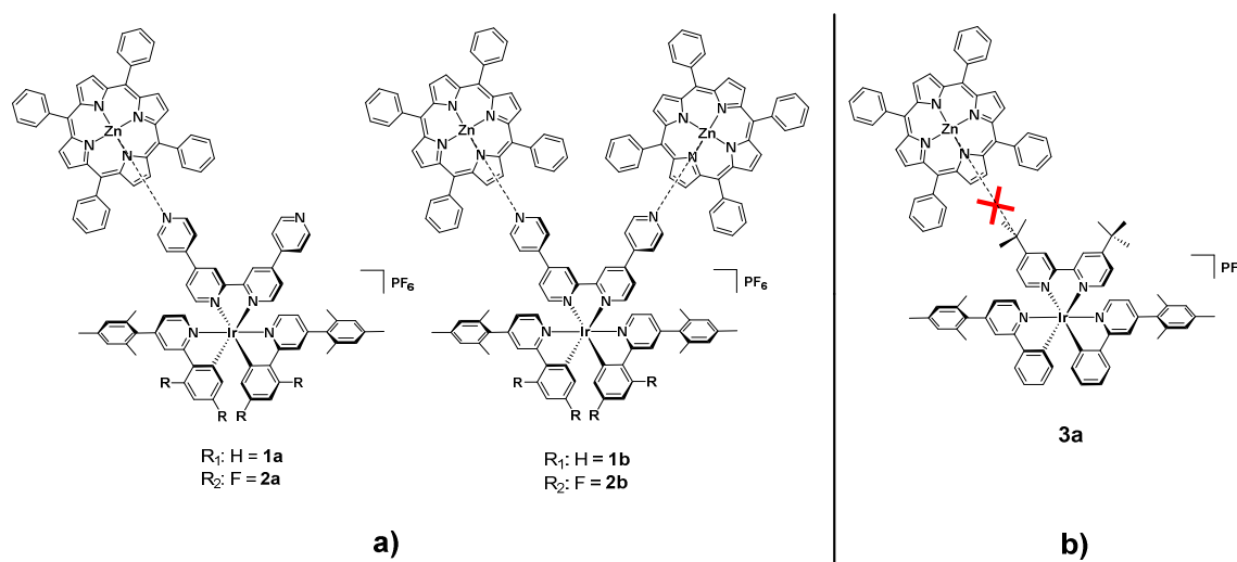
Chart 2. Chemical structures of a ) the assemblies 1a [\text{Ir}(\text{mesppy})_2(\text{qpy})]\text{PF}_6 : ZnTPP 1:1 ratio and 2a [\text{Ir}(\text{dFmesppy})_2(\text{qpy})]\text{PF}_6 : ZnTPP 1:1 ratio; 1b [\text{Ir}(\text{mesppy})_2(\text{qpy})]\text{PF}_6 : ZnTPP 1:2 ratio and 2b [\text{Ir}(\text{dFmesppy})_2(\text{qpy})]\text{PF}_6 : ZnTPP 1:2 ratio, and b ) Chemical structure of complex 3 mixed with ZnTPP ( 3a ) used as a control experiment.
