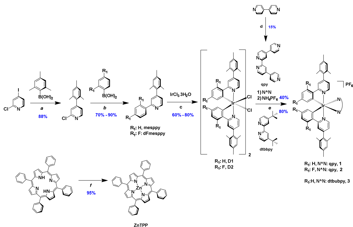
Scheme 1. Synthesis of C ^ N and qpy ligands and [Ir(C ^ N) 2 (N ^ N)]PF 6 complexes 1 , 2 and 3 .
