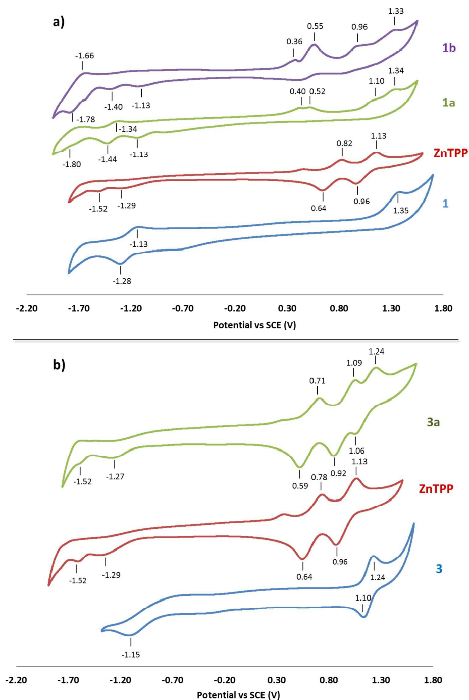
Figure 8. a) CVs for 1 , ZnTPP , 1a and 1b and b) CVs for 3 , ZnTPP and 3a recorded at 298 K in deaerated DCM solution containing n\text{-NBu}_4\text{PF}_6 as the supporting electrolyte and using \text{Fc}/\text{Fc}^+ as an internal standard ( \text{Fc}/\text{Fc}^+ = 0.46 V in DCM with respect to SCE). 30
