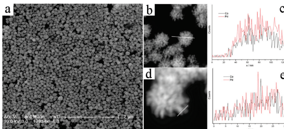
Figure 5. (a) SEM image of \text{CoPd}_2 nanocrystals; (b and d) HAADF-STEM images of \text{CoPd}_2 nanocrystals. (c) The elemental profiles for Co and Pd obtained by recording EDS signal intensities along the line shown in part b; (e) the elemental profiles for Co and Pd obtained by recording EDS signal intensities along the line shown in part d.
