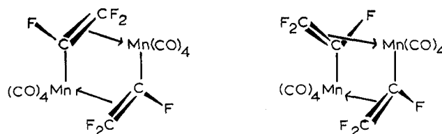
Figure 1.—Isomeric forms of [\text{CF}_2=\text{CFMn}(\text{CO})_4]_2 .
