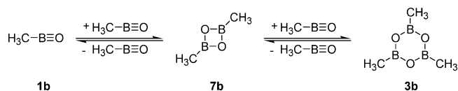
Scheme 4. Stepwise Trimerization of Methyl(oxo)borane 1b To Give Trimethylboroxin 3b
