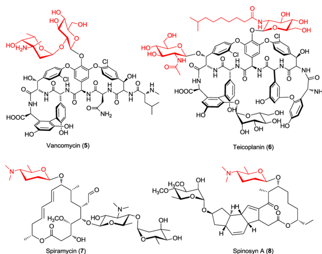
Figure 2. Structures of the natural glycopeptide antibiotics vancomycin ( 5 ) and teicoplanin ( 6 ) and known natural products containing D-forosamine.
