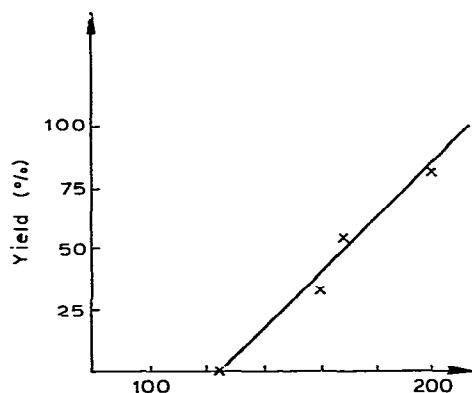
Fig. 1. \alpha\text{-NpPhSiH}_2 + menthol/ \text{HCO}_2\text{K} (m.p. 167^\circ\text{C} ) 3 h at different temperatures. Product: \alpha -naphthyl-phenylmenthoxyasilane.
