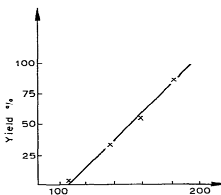
Fig. 1. \alpha\text{-NpPhSiH}_2 + menthol/ \text{HCO}_2\text{K} (m.p. 167^\circ\text{C} ) 3 h at different temperatures. Product: \alpha -naphthyl-phenylmenthoxyasilane.
