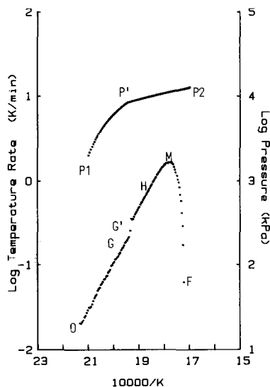
Fig. 1. Experimental ARC results for the titanium-surface-catalyzed decomposition of hydrazine. Segment O-F is the log(temperature rate), left-hand scale. Segment P1-P2 is the log(pressure), right-hand scale.
