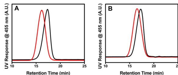
Figure 2. Size exclusion chromatograms of polymers obtained via chain extension. (A) PPE homopolymer before (black line; M_n = 10 500 Da, \bar{D} = 1.40) and after (red line; M_n = 23 700 Da, \bar{D} = 1.48) adding a second feed of 2 . (B) PPE macroinitiator (black line; M_n = 10 500 Da, \bar{D} = 1.39) and corresponding PPE- b -poly(fluorenylethynylene) block copolymer (red line; M_n = 16 000 Da, \bar{D} = 1.55).
