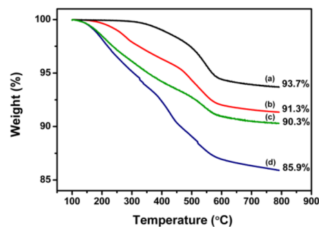
Figure 4. TGA curves of (a) bare SiO 2 particles, (b) SiO 2 -PhBr , (c) SiO 2 -Pd , and (d) SiO 2 -PPE . The TGA experiments were performed under an atmosphere of nitrogen at a heating rate of 20^\circ\text{C min}^{-1} .
