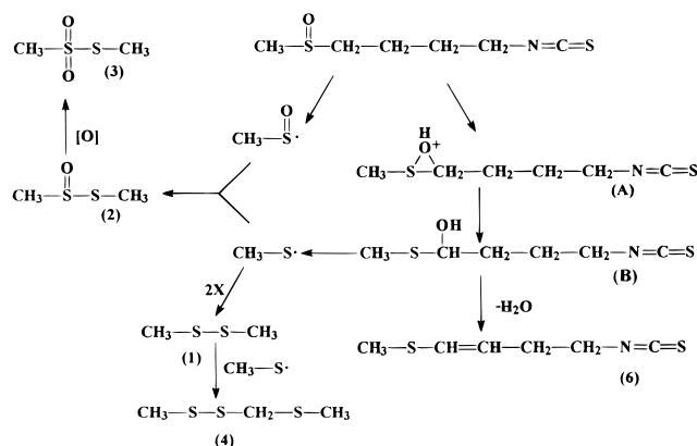
Figure 1. Possible pathways for the formation of volatile compounds generated from thermal degradation of sulforaphane [1, dimethyl disulfide; 2, S-methyl methylthiosulfinate; 3, S-methyl methylthiosulfonate; 4, methyl (methylthio)-methyl disulfide; 6, 4-isothiocyanato-1-(methylthio)-1-butene].
