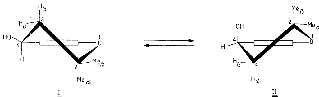
Fig. 1. Conformations I and II of the tetrahydropyran ring
