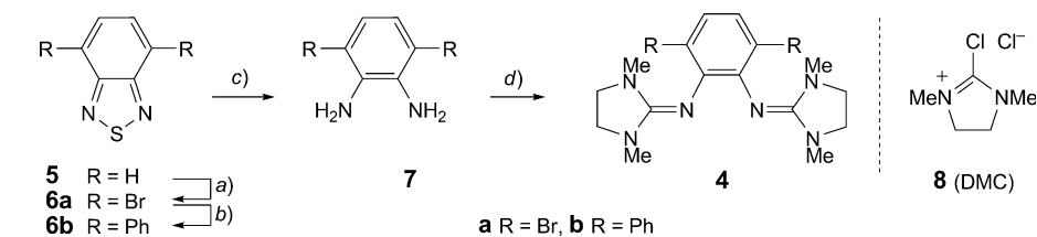
Scheme 1. Synthesis of 3,6-Disubstituted BGs 4a and 4b
