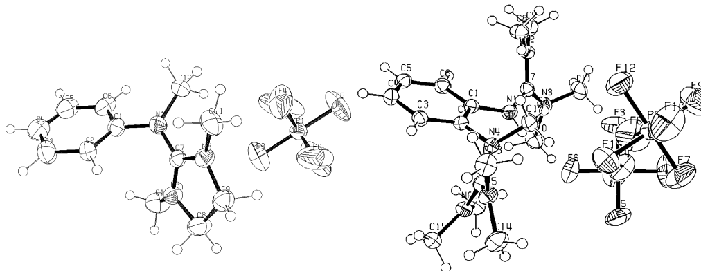
Fig. 9. ORTEP Plots of 19e (left) and 21 (right)
