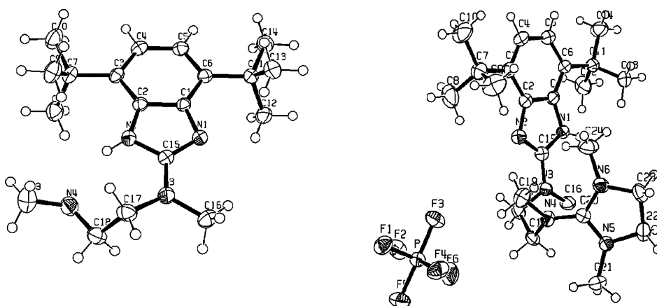
Fig. 3. ORTEP Plots of 14 (left) and 16 (right)
