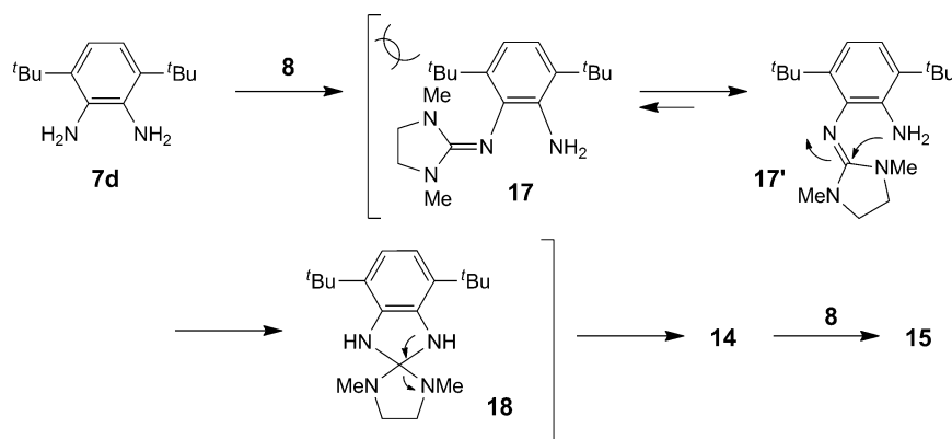
Scheme 3. Proposed Mechanism of the Generation of 14 and 15 from 7d
