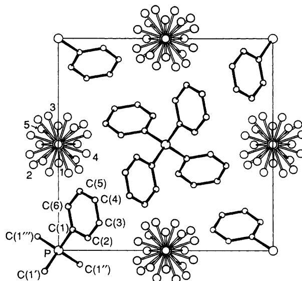
Fig. 2 Projection down the c axis of a cell of [\text{PPh}_4][\text{VO}_2\text{F}_2] . The P atom lies at the origin from which the a axis goes up the page and the b axis to the right across the page. In the anion the number of the oxygen/fluorine atom is indicated; O/F(6) lies directly above the V atom
