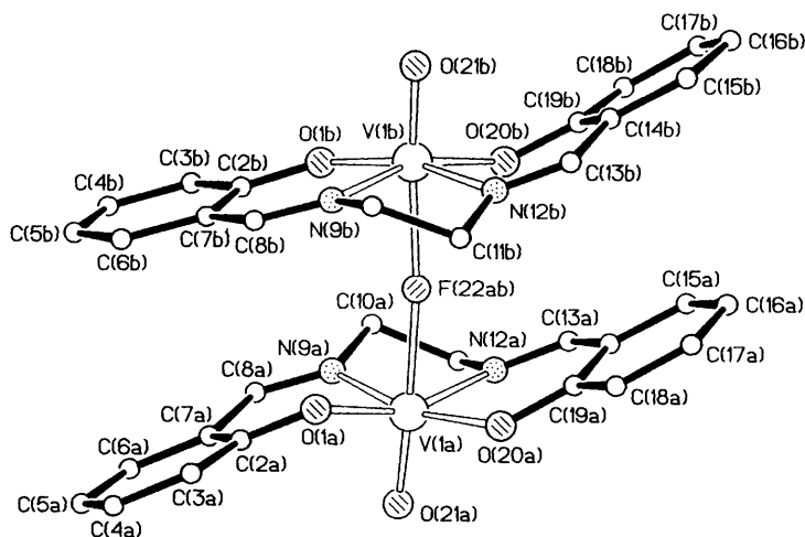
Fig. 1 One of the two independent, virtually identical cations in [\{\text{VO}(\text{salen})\}_2(\mu\text{-F})][\text{BF}_4] , showing the atom numbering scheme
