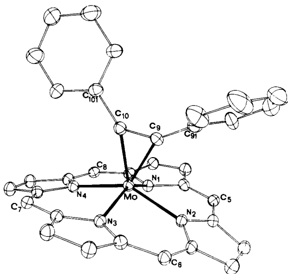
Figure 1. ORTEP drawing of \text{Mo}(\text{TTP})(\text{PhC}\equiv\text{CPh}) . All atoms are represented by 50% probability thermal ellipsoids. For clarity the phenyl groups of the porphyrin were omitted. Main distances (Å) are Mo–N 1 , 2.104 (3); Mo–N 2 , 2.150 (3); Mo–N 3 , 2.105 (3); Mo–N 4 , 2.147 (3); Mo–C 9 , 1.983 (4); Mo–C 10 , 1.965 (4); C 9 –C 10 , 1.324 (5); C 10 –C 101 , 1.485 (5); C 9 –C 91 , 1.455 (5). Main angles (deg) are N 1 –Mo–N 4 , 85.1 (1); N 2 –Mo–N 4 , 145.1 (1); N 2 –Mo–N 3 , 85.2 (1); N 3 –Mo–N 4 , 84.6 (1); C 9 –C 10 –C 101 , 136.4 (4); C 10 –C 9 –C 91 , 145.4 (4).
