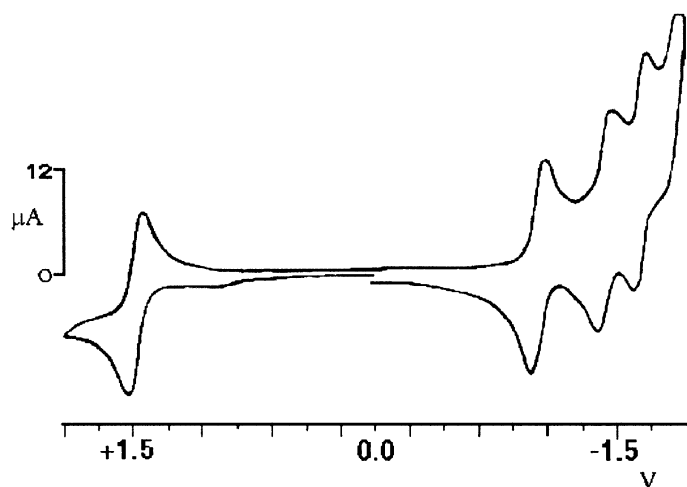
Fig. 4. Cyclic voltammogram of [\text{Ru}(\text{bpy})_2((\text{COOMe})\text{ppl})](\text{PF}_6)_2 ( 12 ) in MeCN
