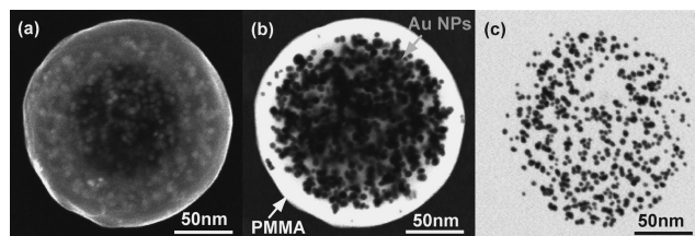
Figure 3. A SEM mode (a), a dark field STEM mode (b) image, and a cross-sectional TEM image (c) of a core-shell type nanocomposite particle.
