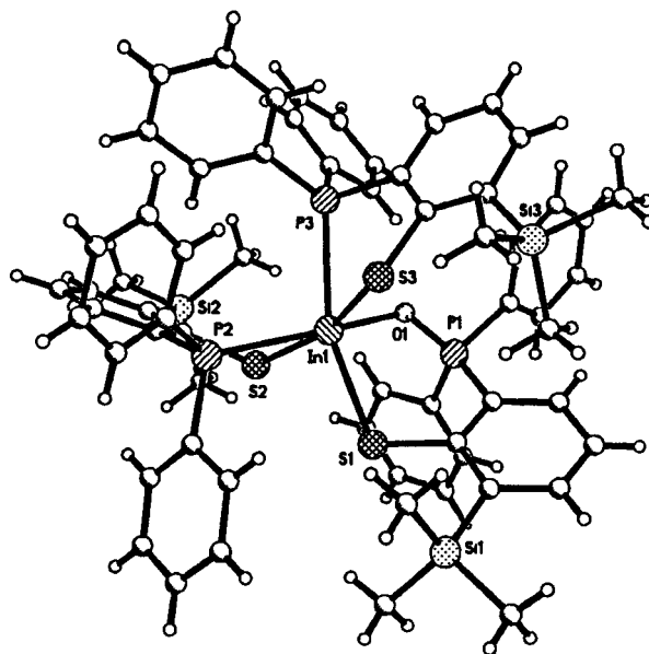
Figure 2. View of the structure of [\text{In}\{2\text{-(Ph}_2\text{P)-6-(Me}_3\text{Si)C}_6\text{H}_3\text{S}\}_2\{2\text{-(Ph}_2\text{PO)-6-(Me}_3\text{Si)C}_6\text{H}_3\text{S}\}] (2), showing the atom-labeling scheme and 50% thermal ellipsoids.
