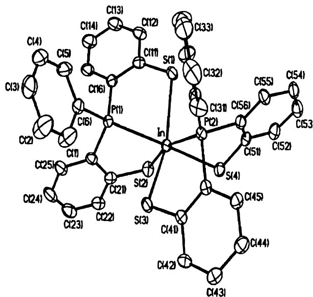
Figure 3. View of the structure of the anion [\text{In}\{\text{PhP(C}_6\text{H}_4\text{S-2)}_2\}_2]^- of 4, showing the atom-labeling scheme and 50% thermal ellipsoids.
