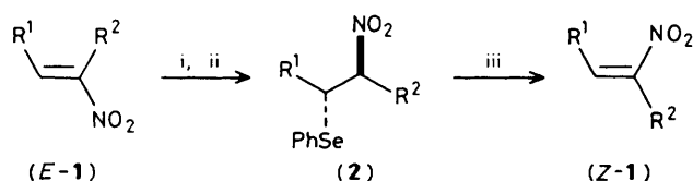
Scheme 1. Reagents: i, PhSeNa (1.2 equiv.), EtOH, -78^{\circ}\text{C} , 1 h; ii, AcOH (2 equiv.), -78^{\circ}\text{C} , 1 h; iii, H 2 O 2 (30%), CH 2 Cl 2 , 0^{\circ}\text{C} , 10 min.
