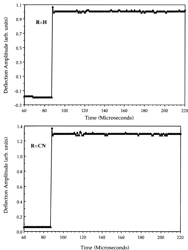
Figure 4. Time-resolved photothermal beam deflection signal generated from pulsed laser photolysis of 1a (top panel) and 1g (bottom panel) in Ar-purged CH 3 CN. Excitation pulse arrived at ca. 88 \mu s on the time axis shown.
