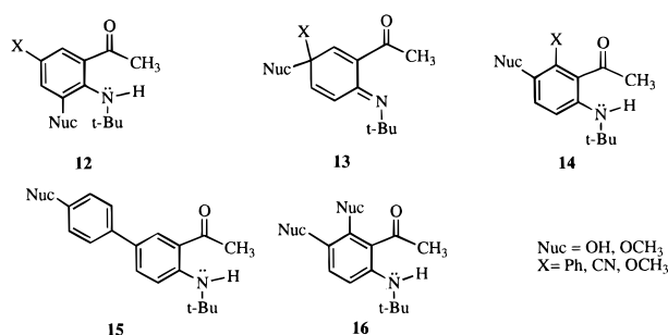
Chart 1. Nucleophilic Addition Products
