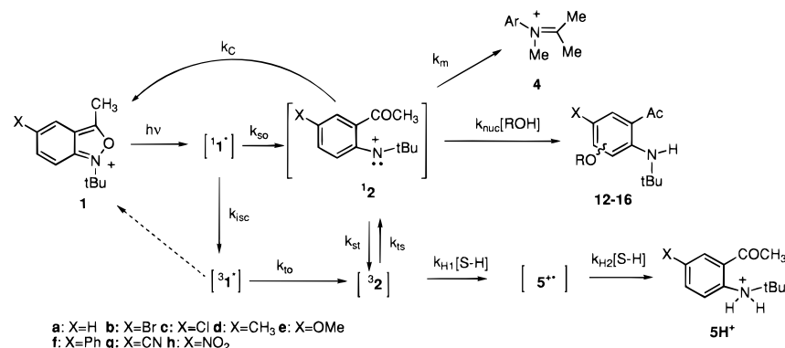
Chart 1. Nucleophilic Addition Products
