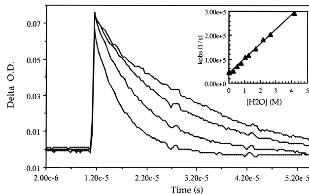
Figure 2. Decay waveforms from laser flash photolysis of 1f in CH 3 CN containing 0.00–4.17 M H 2 O monitored at 470 nm, the absorption maximum of the arylnitrenium ion 2f (see Figure 1 and text). Inset shows the dependence of the pseudo-first-order decay rate constant, k_{\text{obs}} on [H 2 O].
