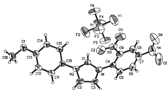
Fig. 1 Single-crystal X-ray crystal structure of 3d .
