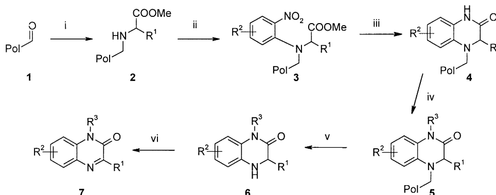
Scheme 1. Traceless synthesis of quinoxalinones. Reagents: (i) amino acid ester, \text{NaB}(\text{AcO})_3\text{H} , DMF/AcOH; (ii) o -fluoronitrobenzene, DMSO, 75°C, 1–3 days, see Table 1; (iii) \text{SnCl}_2 \cdot 2\text{H}_2\text{O} , NMP, rt, 2 h; (iv) 2- t -butyl-imino-2-diethylamino-1,3-dimethylperhydro-1,3,2-diazaphosphorine (BEMP), alkyl halide, DMF, rt, 2 h; (v) TFA or gaseous HCl or gaseous HF, rt, 2 h; (vi) air oxidation, MeOH, rt, overnight
