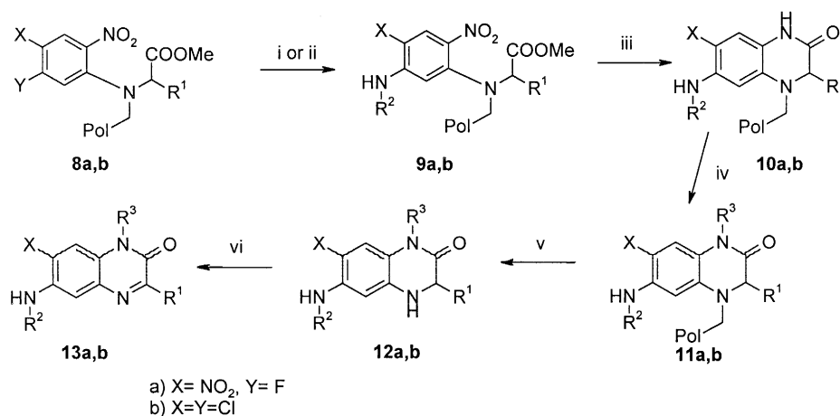
Scheme 2. Extending the diversity of quinoxalinones. Reagents: (i) amine, DMF, rt, overnight; (ii) amine, DMSO, 75°C, overnight; (iii) SnCl 2 ·2H 2 O, NMP, rt, 2 h; (iv) alkyl halide, BEMP, DMF, rt, 2 h; (v) TFA or gaseous HF or HCl, rt, 2 h; (vi) air oxidation, MeOH, rt, overnight
