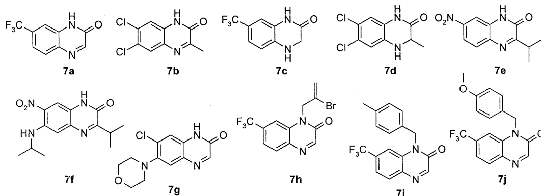
Fig. 1. Structure of representative quinoxalinones
