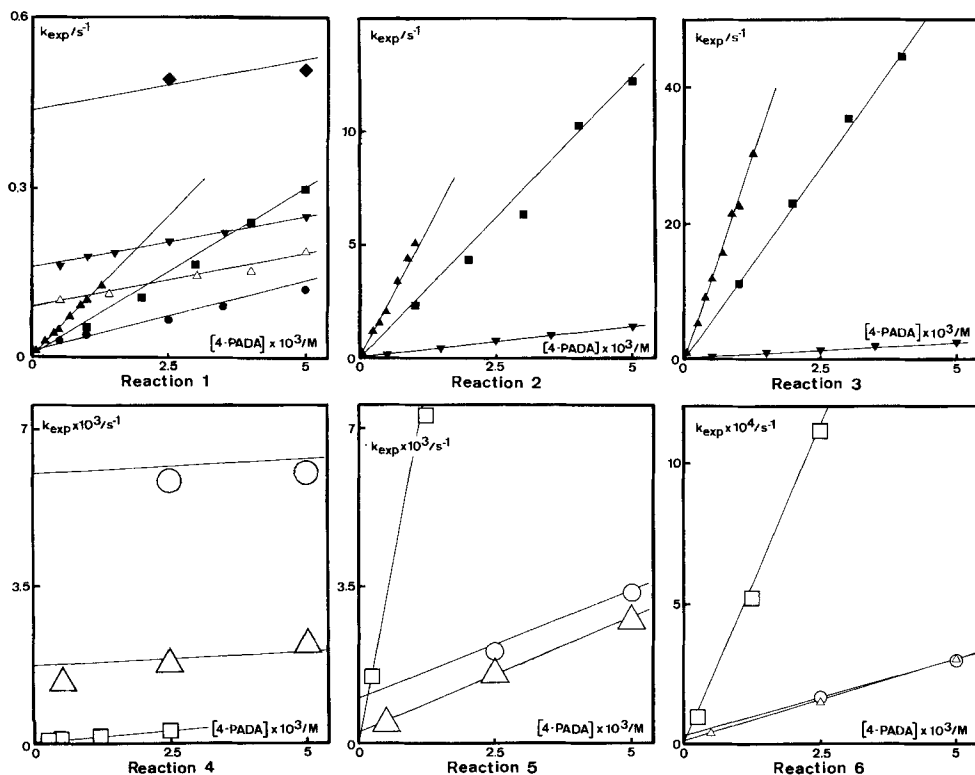
Fig. 2. Plots of k_{\text{exp}} vs. [\text{4-PADA}] for Reactions 1–6. The ratios [\text{Cl}^-]/[\text{4-PADA}] were 12.5/1 (▲), 10/1 (□), 6.25/1 (■), 1/1 (●), 1/10 (△), 1/20 (▼), 1/50 (○), and 1/100 (◆). The straight lines were calculated from Eqn. 14 using the final rate constants in Table 3. For clarity, some series of experiments have been excluded.
