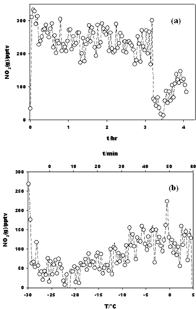
Figure 5. (a) NO 2 (g) concentrations above frozen 2\text{ }\mu\text{M} aqueous nitrate irradiated at -30\text{ }^{\circ}\text{C} for 3.25 h, and then warmed at H = 0.70\text{ }^{\circ}\text{C min}^{-1} in the dark. (b) A blowup of part a after 3.25 h.
