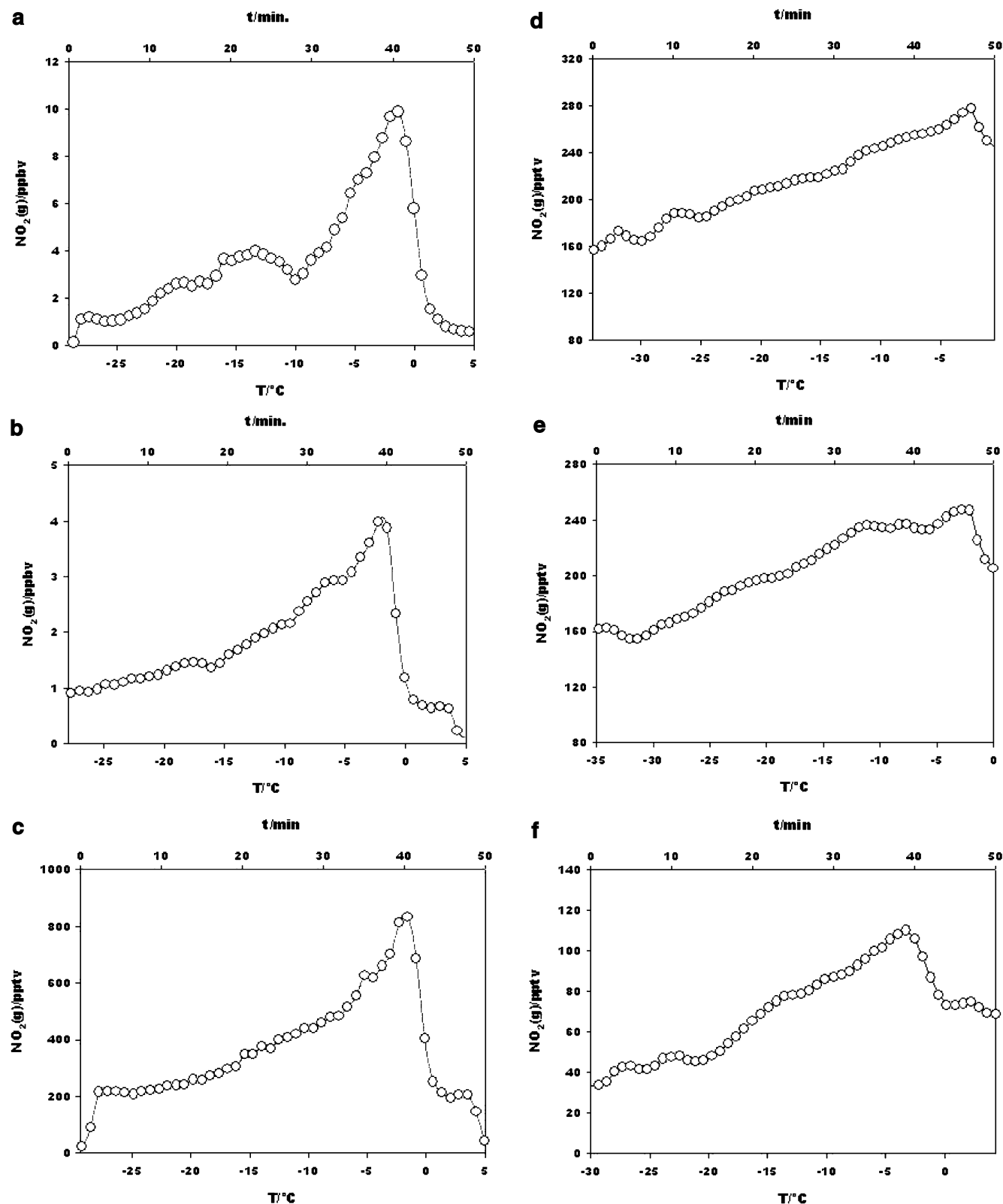
Figure 3. (a) \text{NO}_2(\text{g}) concentration vs temperature during irradiation of frozen 50 mM aqueous nitrate under H = 0.70^\circ\text{C min}^{-1} . (b) \text{NO}_2(\text{g}) concentration vs temperature during irradiation of frozen 10 mM aqueous nitrate under H = 0.70^\circ\text{C min}^{-1} . (c) \text{NO}_2(\text{g}) concentration vs temperature during irradiation of frozen 1 mM aqueous nitrate under H = 0.70^\circ\text{C min}^{-1} . (d) \text{NO}_2(\text{g}) concentration vs temperature during irradiation of frozen 0.2 mM aqueous nitrate under H = 0.70^\circ\text{C min}^{-1} . (e) \text{NO}_2(\text{g}) concentration vs temperature during irradiation of frozen 30 \mu\text{M} aqueous nitrate under H = 0.70^\circ\text{C min}^{-1} . (f) \text{NO}_2(\text{g}) concentration vs temperature during irradiation of frozen 2 \mu\text{M} aqueous nitrate under H = 0.70^\circ\text{C min}^{-1} .
