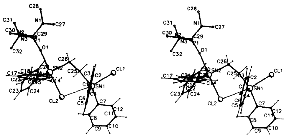
Fig. 2. Stereoscopic view of the molecular structure of (\text{Ph}_2\text{ClSnCH}_2)_2 \cdot \text{HMPA} (7).
