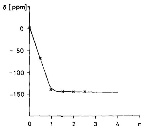
Fig. 1. Plot of the ^{119}\text{Sn} chemical shift of (\text{Ph}_2\text{ClSnCH}_2)_2 \cdot n[\text{Ph}_3\text{P}=\text{N}=\text{PPh}_3]^+ \text{Cl}^- versus n (x marks the experimental values, the solid line represents the calculated Hildebrandt-Benesi equation for a K_a of 2260 \text{ M}^{-1} ).
