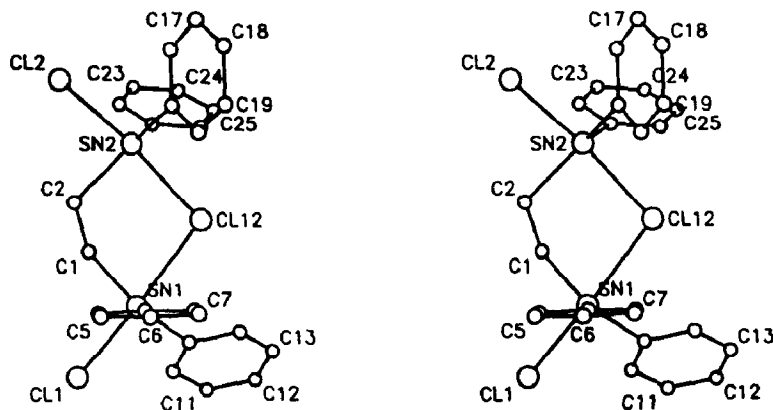
Fig. 3. Stereoscopic view of the molecular structure of [(\text{Ph}_2\text{ClSnCH}_2)_2 \cdot \text{Cl}]^- [\text{Ph}_3\text{P}=\text{N}=\text{PPh}_3]^+ (the cationic part is omitted for clarity).
