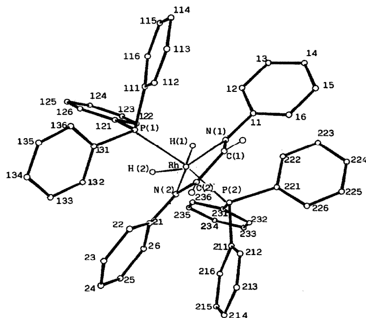
Fig. 1. View of the cationic complex [\text{RhH}_2(\text{Ph-DAB})(\text{PPh}_3)_2]\text{PF}_6 showing the atomic numbering scheme.
