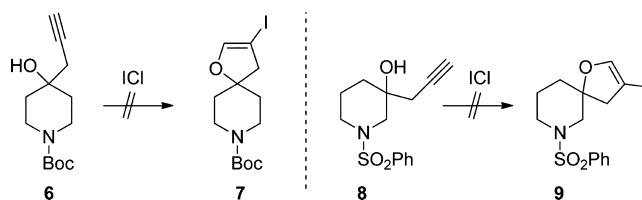
Scheme 3. Attempted Iodoetherification of Homopropargyl Tertiary Alcohols
