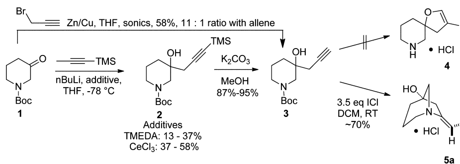
Scheme 1. Synthesis of Bicyclo[3.2.1]- \beta -iodo Enamines from Homopropargyl Tertiary Alcohols Derived from N -Boc-3-piperidone
