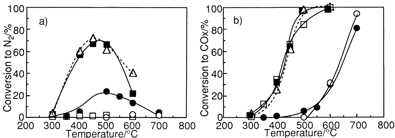
Fig. 1. Reduction of NO by methane over several catalysts as a function of reaction temperature. a) Reduction of NO to N 2 . b) Conversion of methane to CO x .
