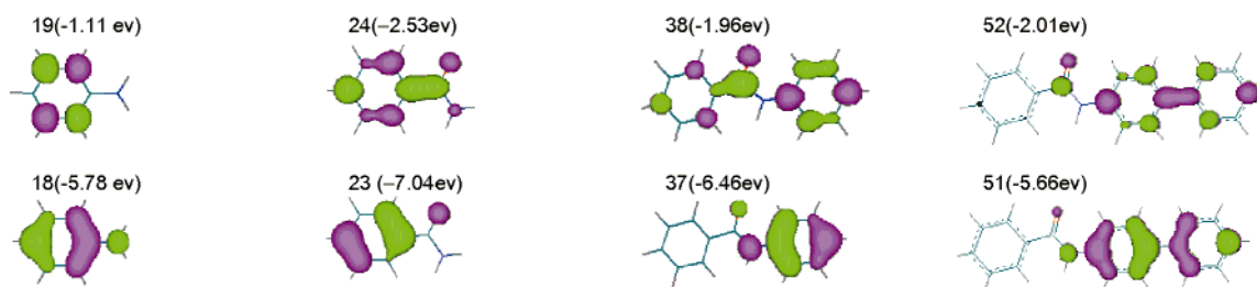
Figure 6. Diagram of frontier orbitals for 1a , 1b , 1 , and 2 .
