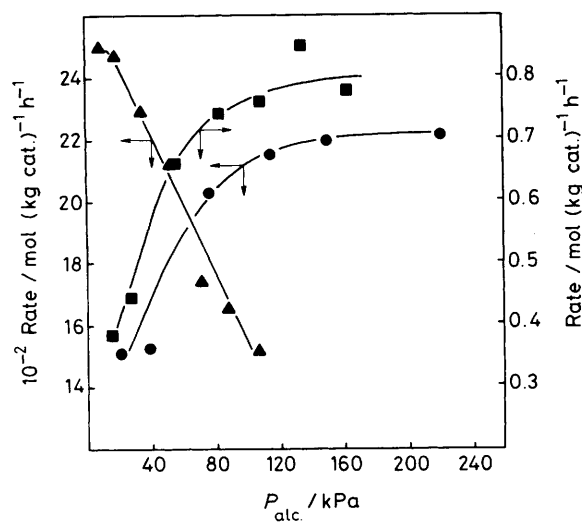
Figure 1. Effect of alcohol partial pressure ( P_{\text{alc.}} ) on the steady state reaction rates. Total pressure, 1.344 \times 10^3 kPa; feed rate of \text{N}_2 + alcohol, 250 \text{ mol (kg cat.)}^{-1} \text{ h}^{-1} ; catalyst (Nafion-H) wt., 2.0 g. ●, MeOH; ■, MeOH-Bu i OH (2:1); ▲, Bu i OH.
