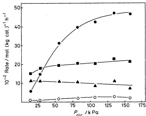
Figure 2. Effect of alcohol mixture (MeOH-Bu i OH, 2:1) partial pressure ( P_{\text{alc.}} ) on the steady-state rates of conversion into: ●, MIBE; ■, Me 2 O; ▲, butenes; ○, Bu i 2 O. Total pressure, 1.344 \times 10^3 kPa; T , 396 K; feed of \text{N}_2 + alcohol, 250 \text{ mol (kg cat.)}^{-1} \text{ h}^{-1} ; catalyst (Nafion-H) wt., 2.0 g.
