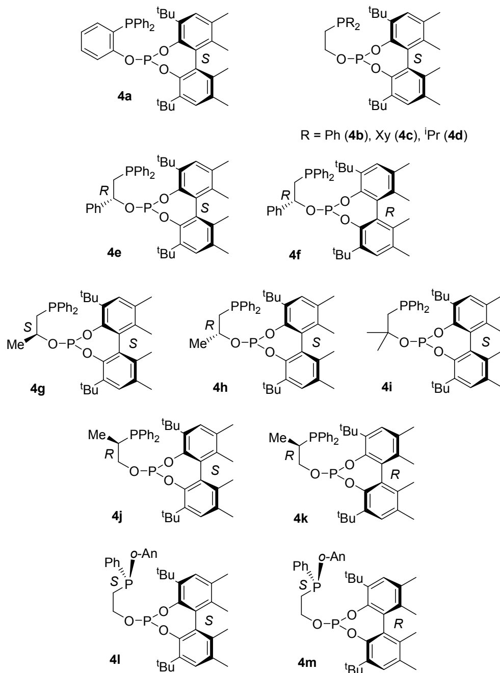
Chart 1. Phosphine-phosphite ligands 4 used in this study.
