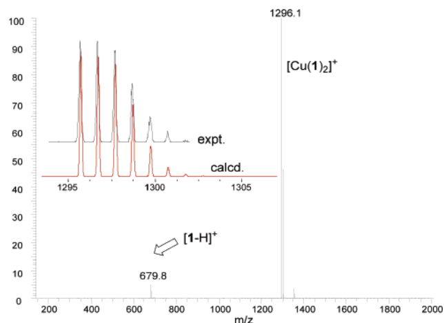
Figure 2. ESI MS of [Cu( 1a ) 2 ] + and its isotopic distribution (dark, experimental; red, calculated). The signal of 1-H + is due to residual traces of acid in the instrument.
