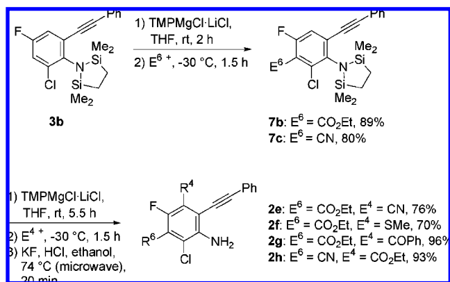
Scheme 4. Polyfunctionalization and Deprotection of p -Fluoro-Substituted Aniline 3b
