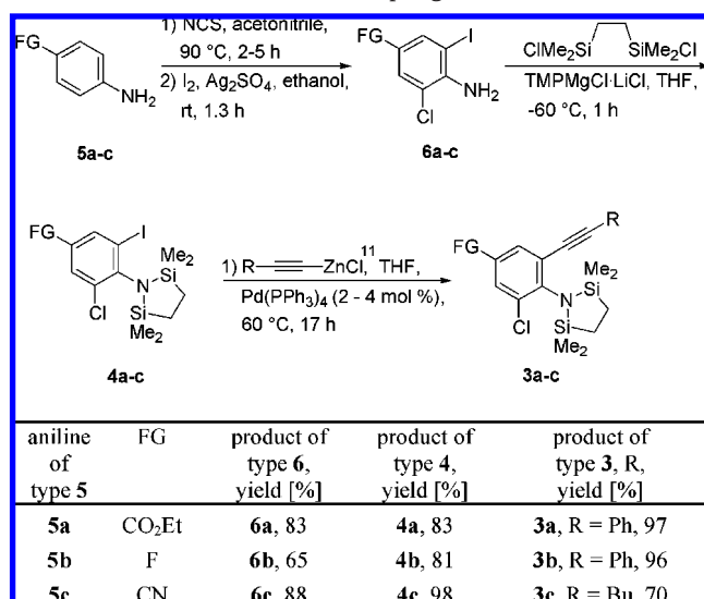
Scheme 2. Selective Halogenation and Protection of Para-Functionalized Anilines of Type 5 Followed by Negishi Cross-Coupling
