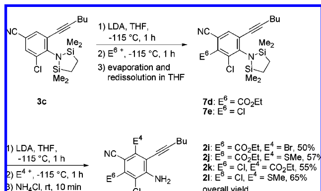
Scheme 5. One-Pot Procedure for the Polyfunctionalization and Deprotection of Aniline Derivative 3c
