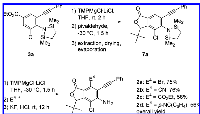
Scheme 3. One-Pot Procedure for the Polyfunctionalization and Deprotection of Aniline Derivative 3a
