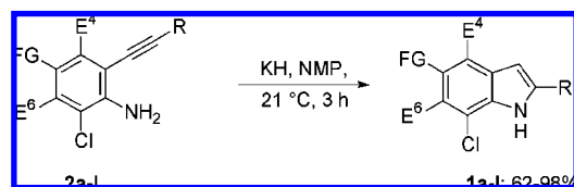
Scheme 6. Potassium Hydride Mediated Cyclization Reaction for the Preparation of Highly Functionalized Indoles 1a–l
