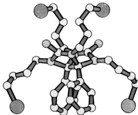
Figure 3. Crystal structure of compound 4a.
