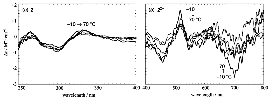
Figure 6. Variable-temperature CD spectra of (a) chiral tetraarylethylene 2 and (b) dication 2^{2+} in 1,2-dichloroethane at -10 , 10 , 30 , 50 , and 70 ^{\circ}\text{C} .
