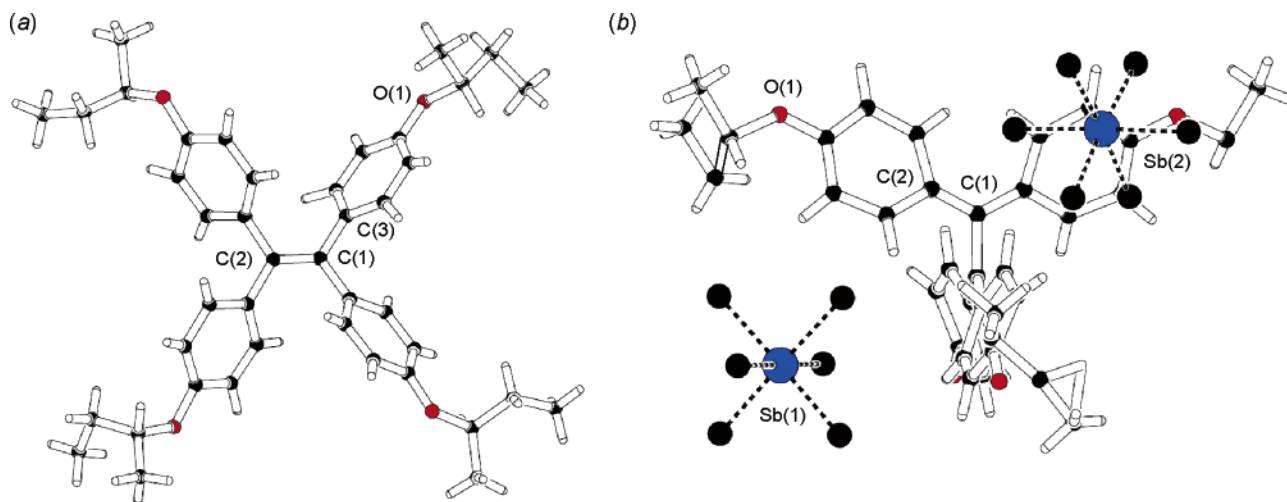
Figure 4. PLUTO drawings of (a) the neutral donor 2 and (b) the corresponding dication 2^{2+}(\text{SbCl}_6^-)_2 . Some atoms are omitted for clarity.
