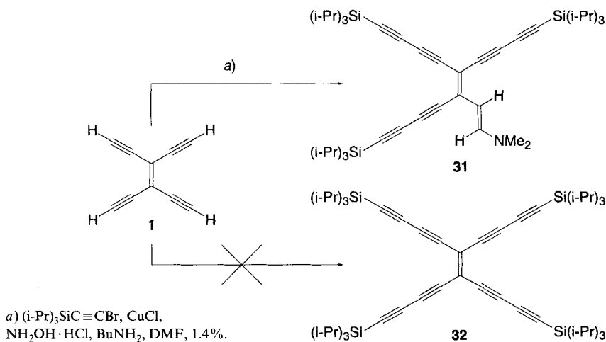
Scheme 5. Attempted Formation of Tetrakis[4-(triisopropylsilyl)buta-1,3-diynyl]ethene ( 32 )
