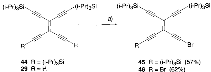
Scheme 7. Synthesis of Brominated Tetraethynylethenes
