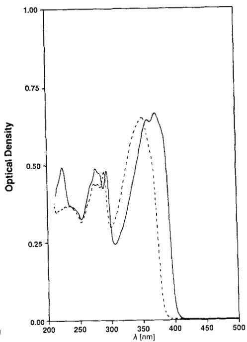
Fig. 3. Electronic absorption spectra of 28 (—) and 30 (----) in \text{MeOH} . T\ 25^\circ , d = 1\text{ cm} , c = 2.09 \cdot 10^{-5}\text{ M} .
