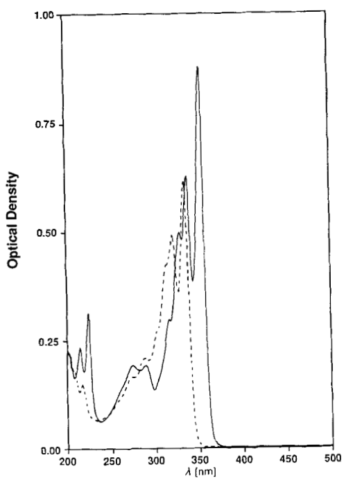
Fig. 2. Electronic absorption spectra of 5 (—) and 1 (----) in \text{MeOH} . T\ 25^\circ , d = 1\text{ cm} , c = 2.33 \cdot 10^{-5}\text{ M} .
