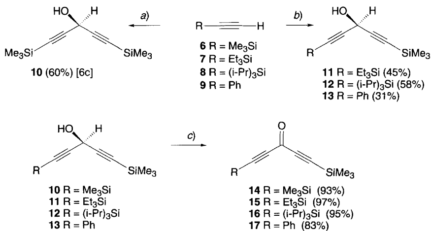
Scheme 2. Syntheses of Penta-1,4-diyn-3-ols and Penta-1,4-diyn-3-ones
