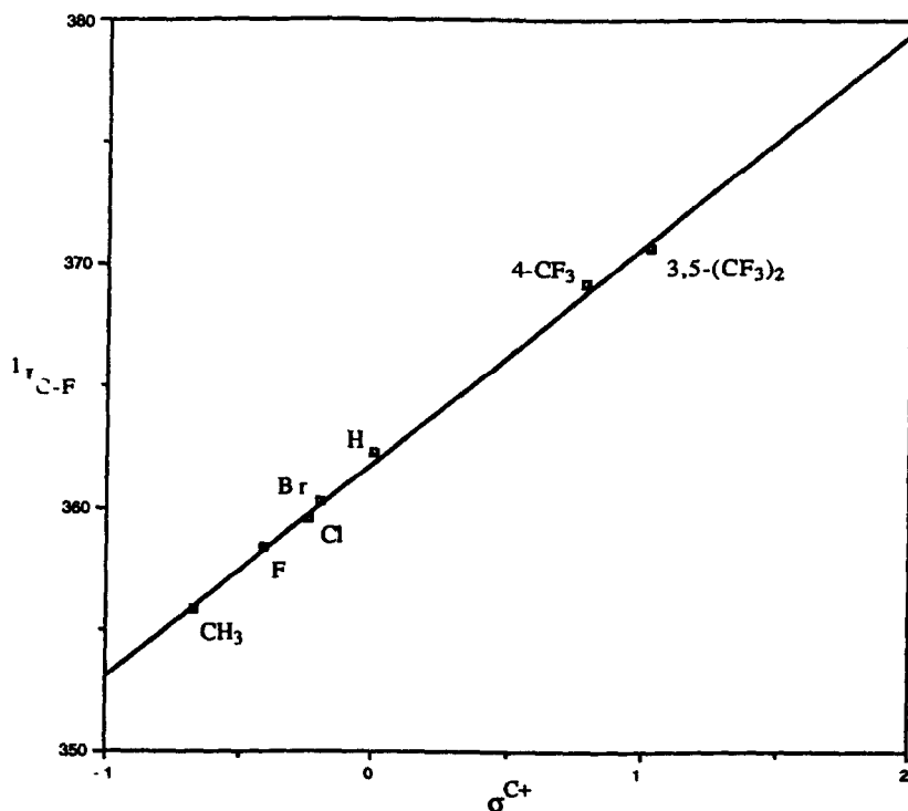
Fig 1 Correlation of one bond ^{13}\text{C} - ^{19}\text{F} coupling constants of \alpha,\alpha -difluoroarylcarbenium ions 1 with \sigma^{C+} substituent constants.
