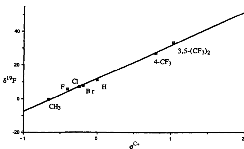
Fig. 2. Correlation of ^{19}\text{F} chemical shifts of \alpha,\alpha -difluoroarylcarbenium ions with \sigma^{C+} substituent constants
