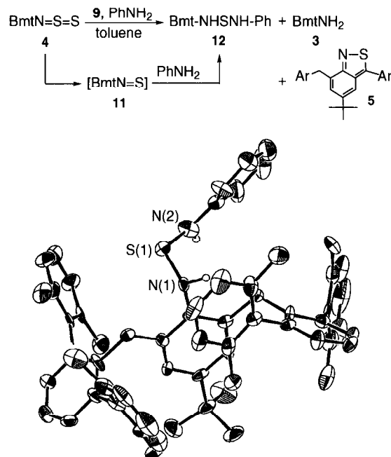
Figure 1. ORTEP drawing of 12 (30% probability).
