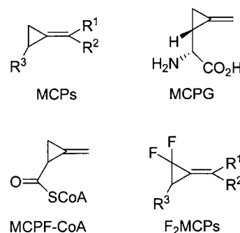
Scheme 1. Structures of various methylenecyclopropanes.
