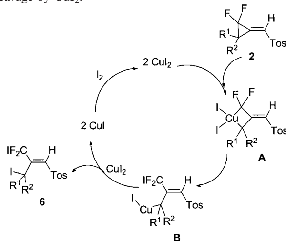
Scheme 2. Proposed mechanism for CuI-promoted ring-opening reactions of F 2 MCPs.
