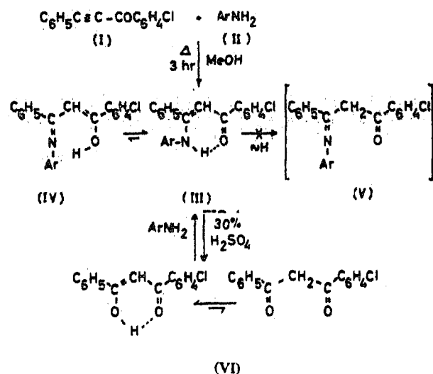
Figure 1. Reaction of ( p -chlorobenzoyl)phenylacetylene with aniline derivatives.
