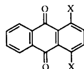
16a, X = OH b, X = NH(CH 2 ) 2 N(CH 3 ) 2 c, X = NH 2
