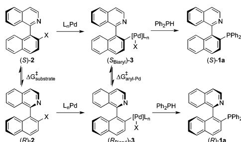
Scheme 1. Kinetic Resolution and DKR Syntheses of QUINAP (1a) (2a–c, 3a–c: X = Br, OTf, OSs)
