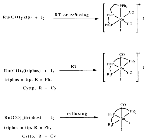
Scheme 1. Reactions of \text{Ru}(\text{CO})_2(\text{triphos}) ( \text{triphos} = \text{etp} , \text{ttp} , and \text{Cytpp} ) with \text{I}_2 in benzene.
