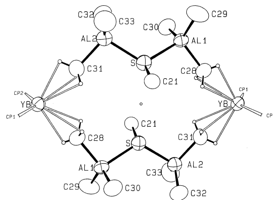
Figure 1. An ORTEP 30 drawing of [(\text{Me}_5\text{C}_5)_2\text{Yb}(\text{AlMe}_3)_2(\text{S-}p\text{-C}_6\text{H}_4\text{Me})]_2\cdot\text{C}_7\text{H}_8 ( 3 ). The toluene of crystallization is not shown. The Yb– \text{Me}_5\text{C}_5 (ring centroid) distance, represented by CP1 which is C(1–5) and CP2 which is C(11–15), is 2.35 Å and the \text{Me}_5\text{C}_5 (ring centroid)–Yb– \text{Me}_5\text{C}_5 (ring centroid) angle is 148°. The p -tolyl ring is represented by its ipso-carbon atom, C(21). The heavy atoms are refined anisotropically and they are shown as 50% probability ellipsoids; the hydrogen atoms on C(28) and C(31) are refined isotropically and they are of arbitrary size.
