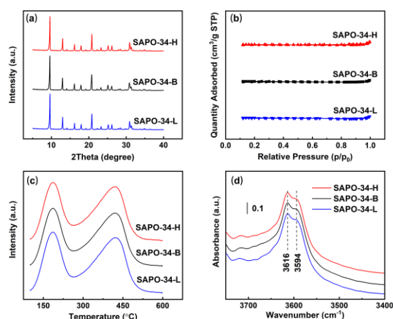
Figure 1. XRD patterns (a), nitrogen adsorption-desorption isotherms (b), NH 3 -TPD profiles (c), and DRIFT spectra (d) of three SAPO-34 samples.
