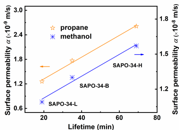
Figure 4. The surface permeability of propane and methanol with regard to the lifetime of SAPO-34 zeolites. The scatters represent the experimental data while solid lines are linearly fitting results.
