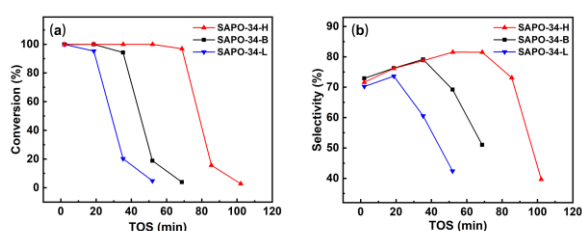
Figure 3. Methanol conversion (a) and light olefins (ethene, propene) selectivity (b) as a function of time on stream (TOS) in MTO reaction over SAPO-34 samples. Reaction condition: 450 °C, methanol WHSV = 5.0 h -1 .
