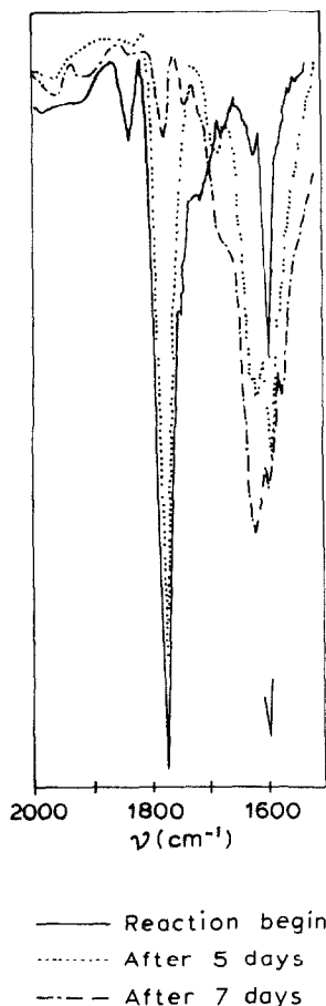
Fig. 1. Reaction of 2f in benzene at room temperature. Change of IR intensities between 2000 and 1500 \text{cm}^{-1} .
