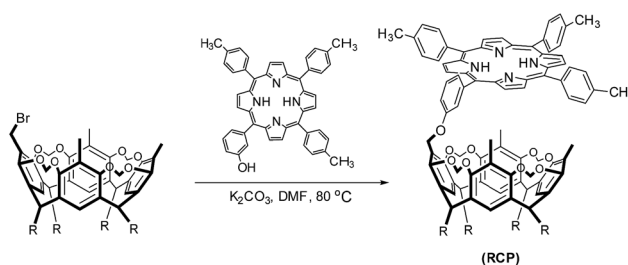
Scheme 1 Synthesis of the cavitand resorcin[4]arene–porphyrin conjugate (RCP).
