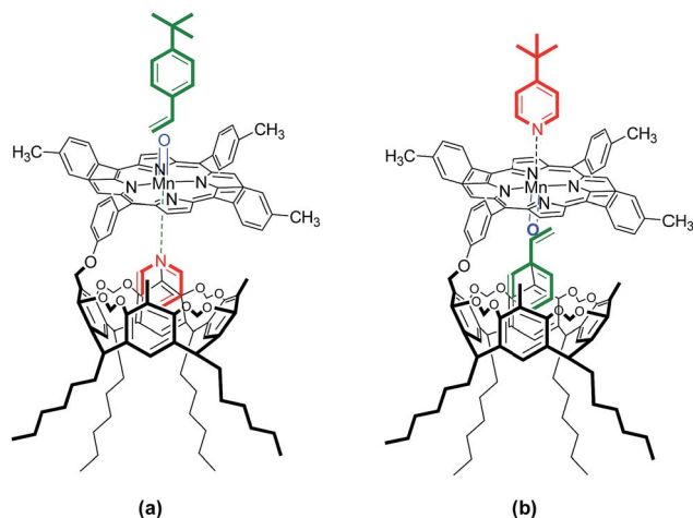
Fig. 6 Representation of the combinations of substrate and axial ligand utilized in the MnRCP-catalyzed epoxidation reactions: (a) pyridine-4- tert -butylstyrene; (b) 4- tert -butylpyridine-styrene.
