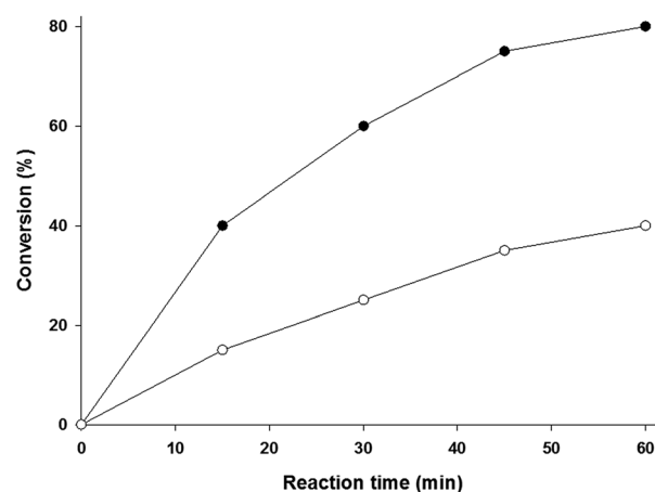
Fig. 9 Plot of percent conversion (%) as a function of reaction time of the epoxidation reaction of t -butylstyrene catalyzed by MnTTP (●) and MnRCP (○) in the presence of t -butylpyridine as an axial ligand.
