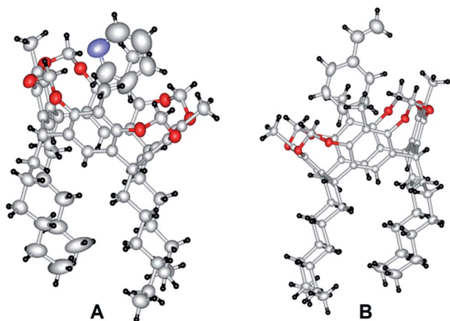
Fig. 4 Thermal ellipsoid representation of the crystal structure of (a) resorcin[4]arene-pyridine (RCPY) and (b) resorcin[4]arene-styrene (RCSTY). Color code: red – oxygen, blue – nitrogen, gray – carbon, black – hydrogen.
