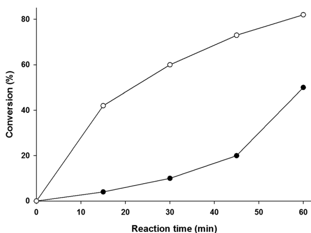
Fig. 7 Plot of conversion (%) as a function of reaction time of the epoxidation reaction of t -butylstyrene catalyzed by MnTTP (●) and MnRCP (○) in the presence of pyridine as an axial ligand.
