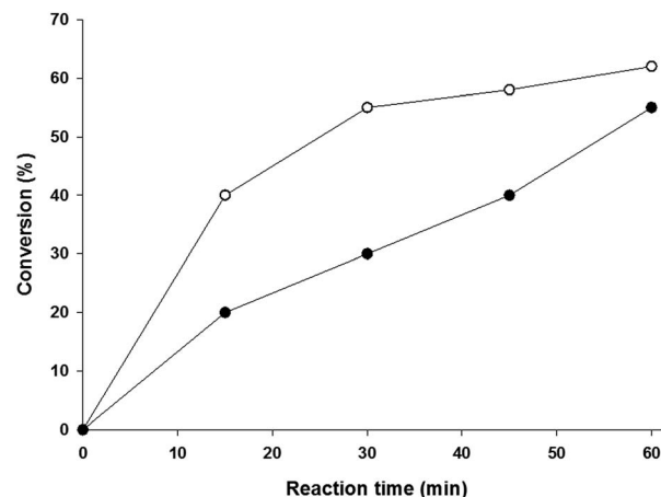
Fig. 8 Plot of conversion (%) as a function of reaction time of the epoxidation reaction of styrene catalyzed by MnTTP (●) and MnRCP (○) in the presence of t -butylpyridine as an axial ligand.
