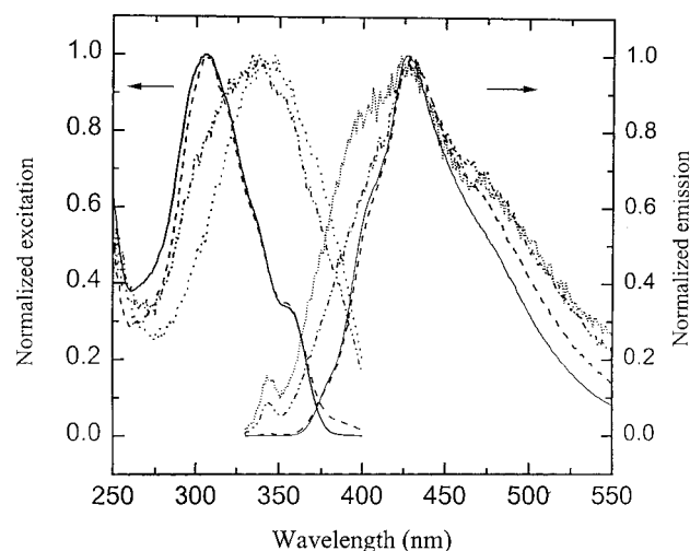
Figure 8. Emission and excitation spectra of TS 4 EPC aqueous dispersion upon photobleaching: — 0 min, --- 16 min, - - - 26 min, ... 36 min.
