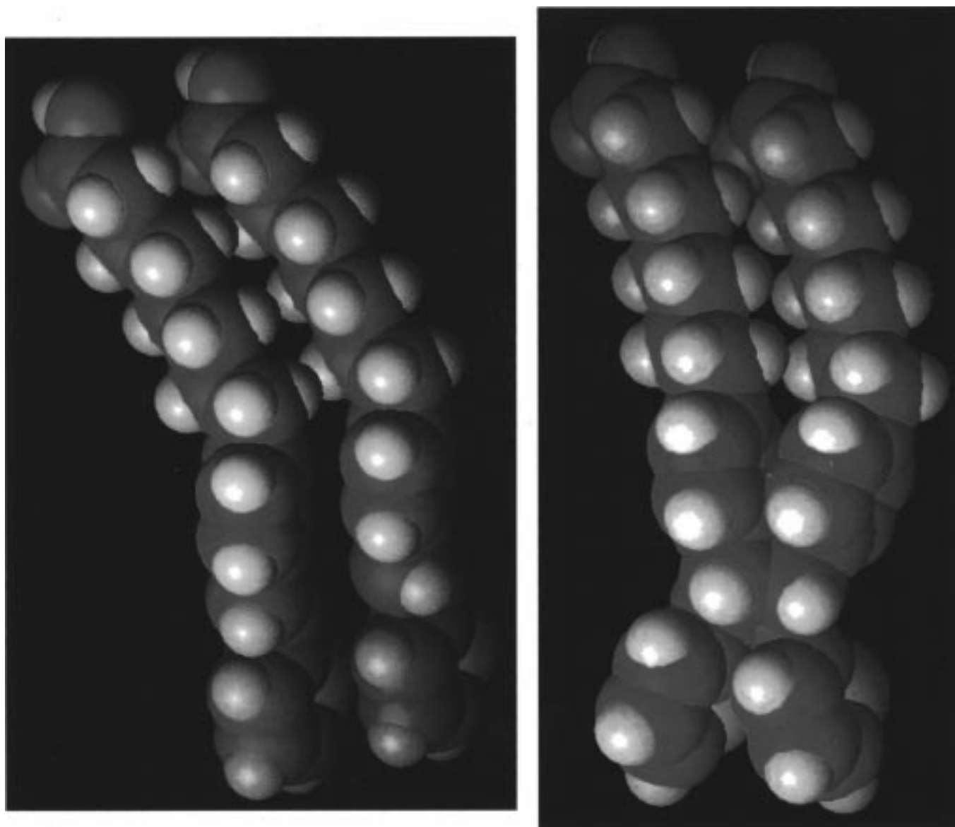
Figure 10. (a, left) Simulated structure of TS 8 A from rank 1 translation layer (Table 3); (b, right) simulated structure of resultant syn-head-head photodimer.
