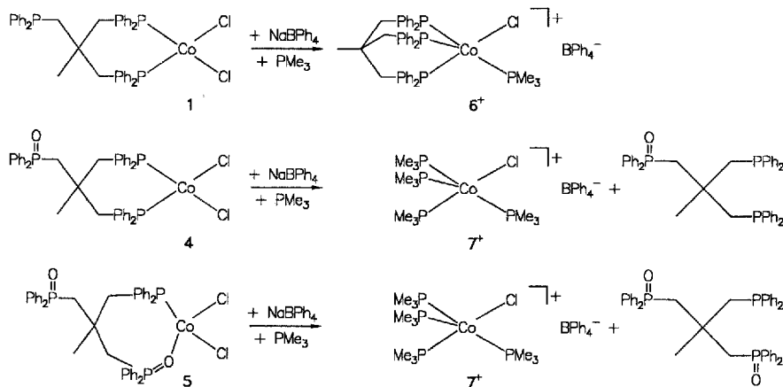
Scheme 5. Reactions of (\text{triphosO}_n)\text{CoCl}_2 with \text{PMe}_3 ( n = 0, 1, 2 )
