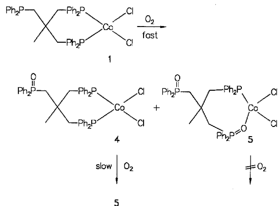
Scheme 3. Reactions of (triphosO n )CoCl 2 with O 2 ( n = 0, 1, 2)
