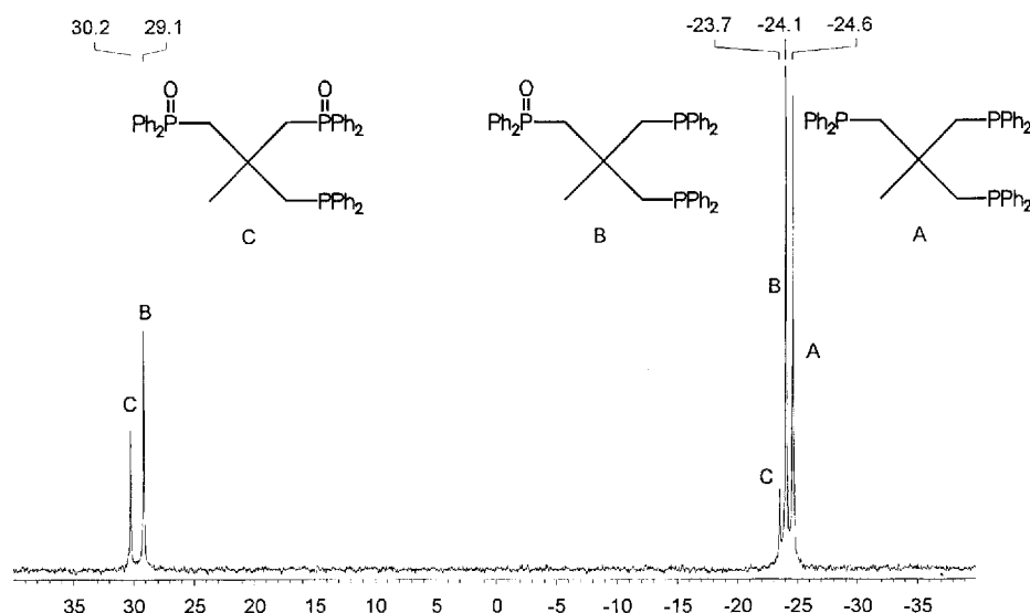
Figure 6. ^{31}\text{P} -NMR spectrum of the products obtained after 2h
