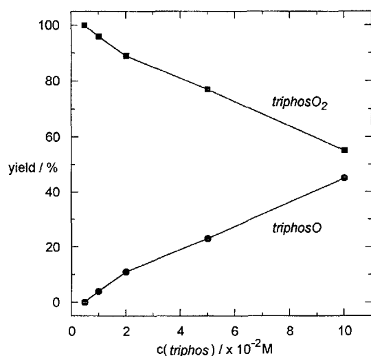
Figure 7. Concentration-dependent product distribution
