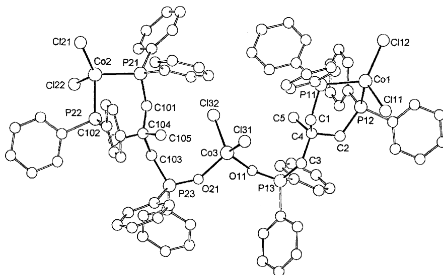
Figure 2. View of the trinuclear unit of (4)_2 \cdot \text{CoCl}_2
