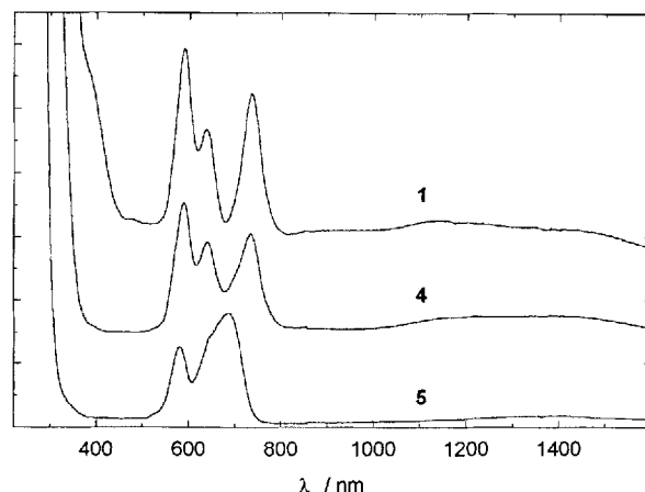
Figure 1. UV/Vis spectra of 1 , 4 and 5 in THF
