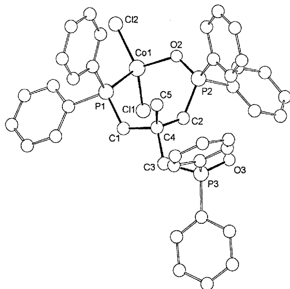
Figure 3. View of the molecular structure of 5 (molecule A)
