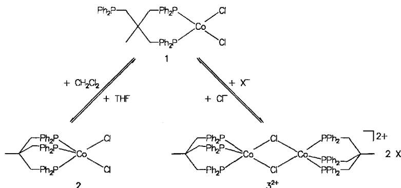
Scheme 1. Complexes of \text{Co}^{\text{II}} with chloride and triphos
