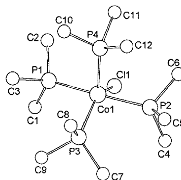
Figure 4. View of the molecular structure of the cation of 7 ·( \text{BPh}_4 )
