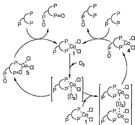
Scheme 7. Proposed catalytic oxygenation cycle of triphos with \text{CoCl}_2
