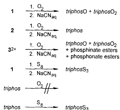
Scheme 2. Reactions with O 2 and S 8
