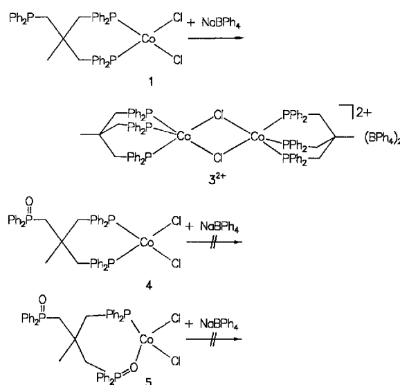
Scheme 4. Reactions of (\text{triphosO}_n)\text{CoCl}_2 with \text{NaBPh}_4 ( n = 0, 1, 2 )
