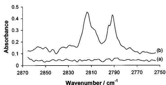
Fig. 2 Infrared spectra of an argon matrix containing \text{CHBr}_2\text{Cl} and \text{O}_3 after (a) deposition and (b) quartz-filtered photolysis ( \lambda > 240 \text{ nm} ) for \approx 120 \text{ h} . Spectrum (b) was recorded at a resolution of 1.0 \text{ cm}^{-1} and shows new bands in the \nu_{\text{H-Cl}} region attributed to the carbon monoxide complexes, \text{OC} \cdots (\text{HCl})_2 , \text{OC} \cdots \text{HCl} , \text{OC} \cdots \text{HCl} \cdots \text{BrCl} , and \text{OC} \cdots \text{BrCl} \cdots \text{HCl} .
