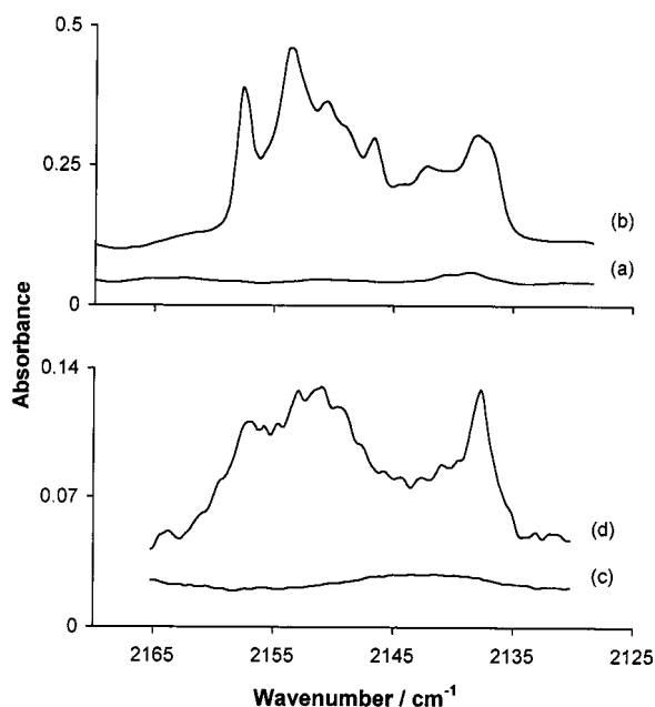
Fig. 4 Infrared spectra recorded after (a) deposition and (b) \approx 120 h of quartz-filtered photolysis ( \lambda > 240 nm) of a \text{CHBr}_2\text{Cl}/\text{O}_3/\text{Ar} matrix. Spectrum (b) was recorded at a resolution of 1.0\text{ cm}^{-1} and shows new bands attributed to \nu_{\text{C=O}} of different carbon monoxide...Lewis acid complexes. Infrared spectra in the \nu_{\text{C=O}} region of a \text{CHBrCl}_2/\text{O}_3/\text{Ar} matrix after (c) deposition and (d) quartz-filtered photolysis for \approx 120 h. Spectrum (d) was recorded at a resolution of 0.5\text{ cm}^{-1} and shows new bands attributed to different carbon monoxide...Lewis acid complexes.
