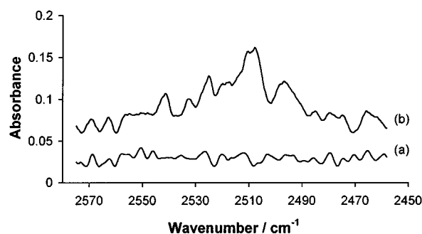
Fig. 3 Infrared spectra recorded after (a) deposition and (b) \approx 120 \text{ h} of quartz-filtered photolysis ( \lambda > 240 \text{ nm} ) of a \text{CHBr}_2\text{Cl}/\text{O}_3/\text{Ar} matrix. Spectrum (b) was recorded at a resolution of 1.0 \text{ cm}^{-1} and shows new bands attributed to \nu_{\text{H-Br}} of different carbon monoxide complexes, \text{OC} \cdots \text{HBr} , \text{OC} \cdots \text{HBr} \cdots \text{Cl}_2 , and \text{OC} \cdots \text{Cl}_2 \cdots \text{HBr} .
